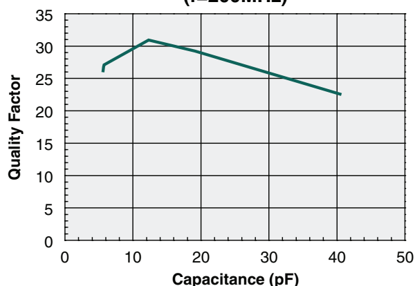
Quality Factor vs. Capacitance TSOT Package (f=200MHz)
