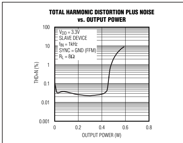
Figure 7. Master-Slave THD+N
