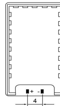
BOTTOM VIEW
