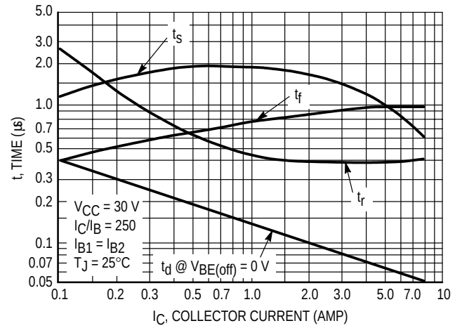
Figure 2. Switching Times
