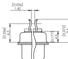
52 Contact design Kontaktvariante Line Contact Termination Kontaktlamellenanschluss
