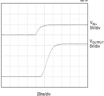
INPUT VOLTAGE vs. OUTPUT VOLTAGE (V + = +16V, C L = 5000pF)
