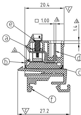
SECTION P-P
