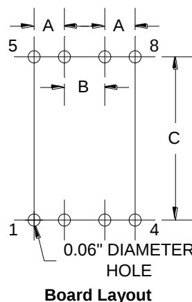
Board Layout
