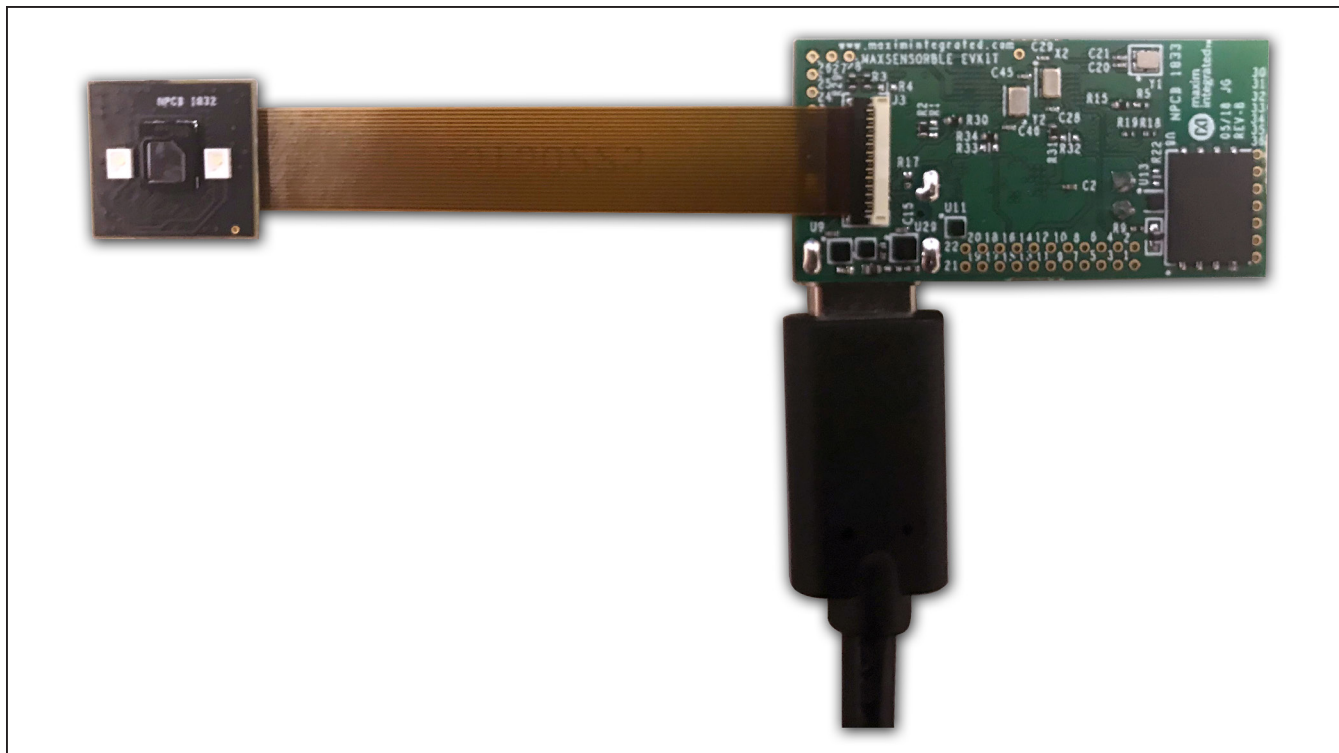
Figure 10. Hardware Setup (MAX86140 EVSYS Sensor PCB)
