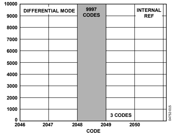
Figure 12. Histogram of Codes for 10,000 Samples @ V_{DD} = 5\text{ V} with Internal Reference
