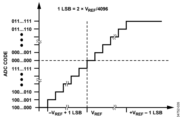
Figure 17. Ideal Transfer Characteristic with Twos Complement Output Coding and 2 \times V_{REF} Range
