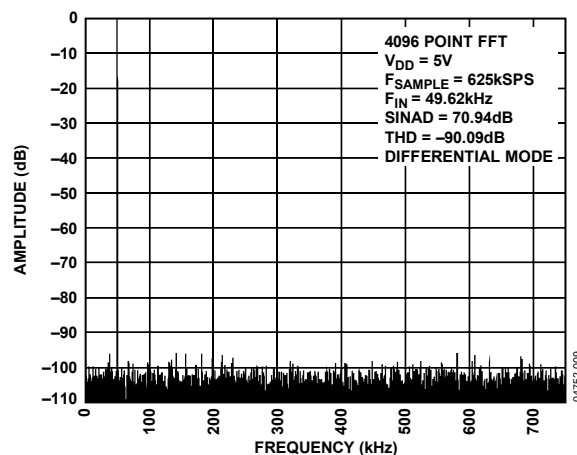
Figure 6. FFT @ V_{DD} = 5\text{V}
