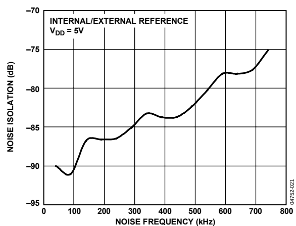
Figure 4. Channel-to-Channel Isolation
