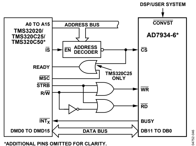
Figure 43. Interfacing to the TMS32020/TMS320C25/TMS320C5x
