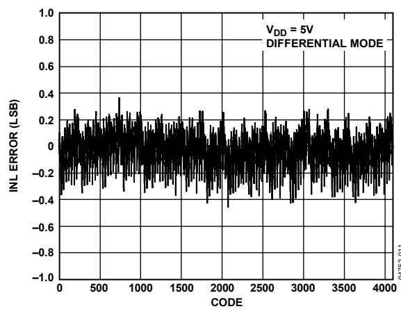
Figure 8. Typical INL @ V_{DD} = 5\text{V}
