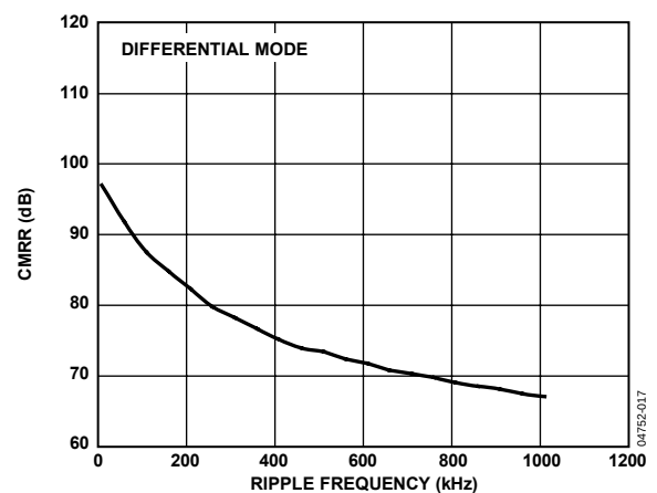
Figure 13. CMRR vs. Ripple Frequency with V_{DD} = 5\text{ V} and 3\text{ V}
