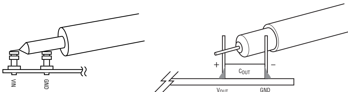
Figure 2. Measuring Input or Output Ripple Across Terminals or Directly Across Bulk Capacitor
