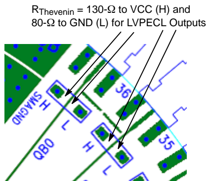
Figure 5. LVPECL Output Configuration, Thevenin Termination Resistors
