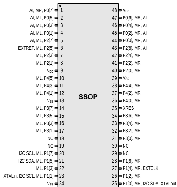
Figure 4. CY8C21645 and CY8C22645 48-pin PSoc Device
