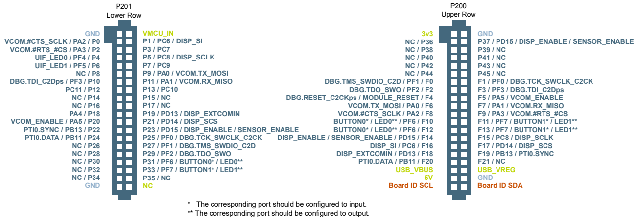
Figure 2.1. BRD4306B Radio Board Connector Pin Mapping
