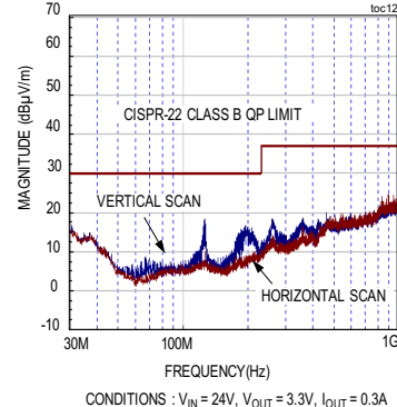
RADIATED EMISSION PLOT (C6 = 0.1µF, C7, C8, C9 = OPEN, L1 = SHORT)
