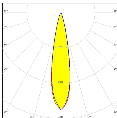
CP16107_CARMEN-50-S-C
