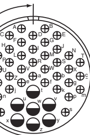
100° Rotation of 36-7
