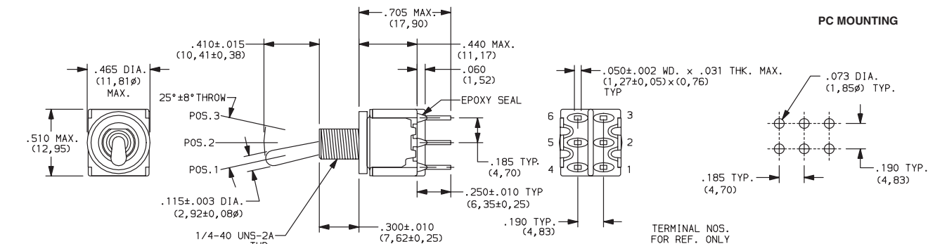
DPDT
