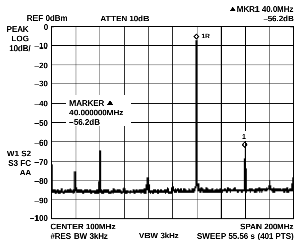
Figure 7. F_{OUT} = 120\text{ MHz} , F_{CLK} = 400\text{ MSPS} , WBSFDR
