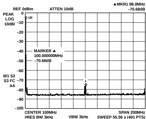
Figure 3. F_{OUT} = 1\text{ MHz} , F_{CLK} = 400\text{ MSPS} , WBSFDR
