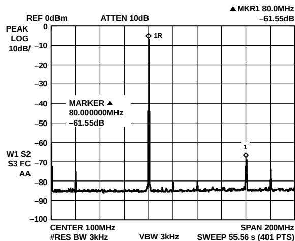
Figure 6. F_{OUT} = 80\text{ MHz} , F_{CLK} = 400\text{ MSPS} , WBSFDR
