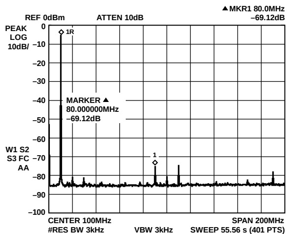
Figure 4. F_{OUT} = 10\text{ MHz} , F_{CLK} = 400\text{ MSPS} , WBSFDR
