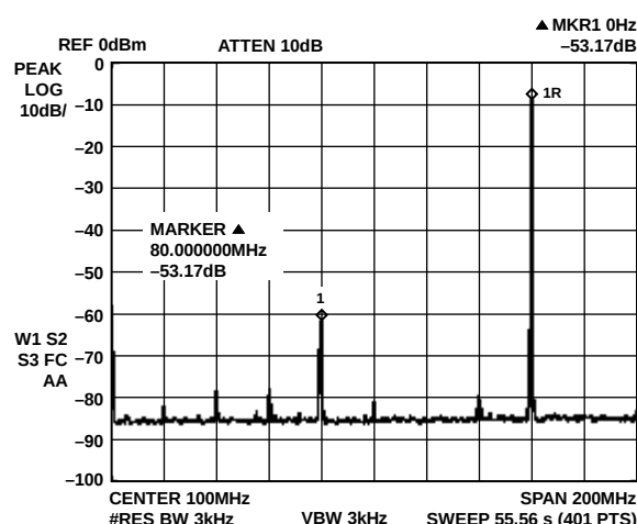
Figure 8. F_{OUT} = 160\text{ MHz} , F_{CLK} = 400\text{ MSPS} , WBSFDR
