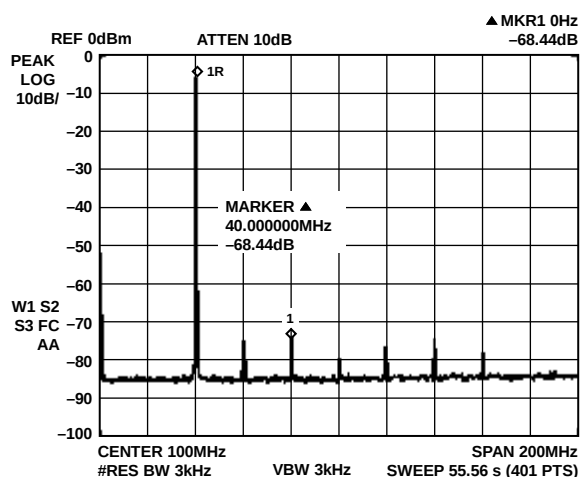
Figure 5. F_{OUT} = 40\text{ MHz} , F_{CLK} = 400\text{ MSPS} , WBSFDR
