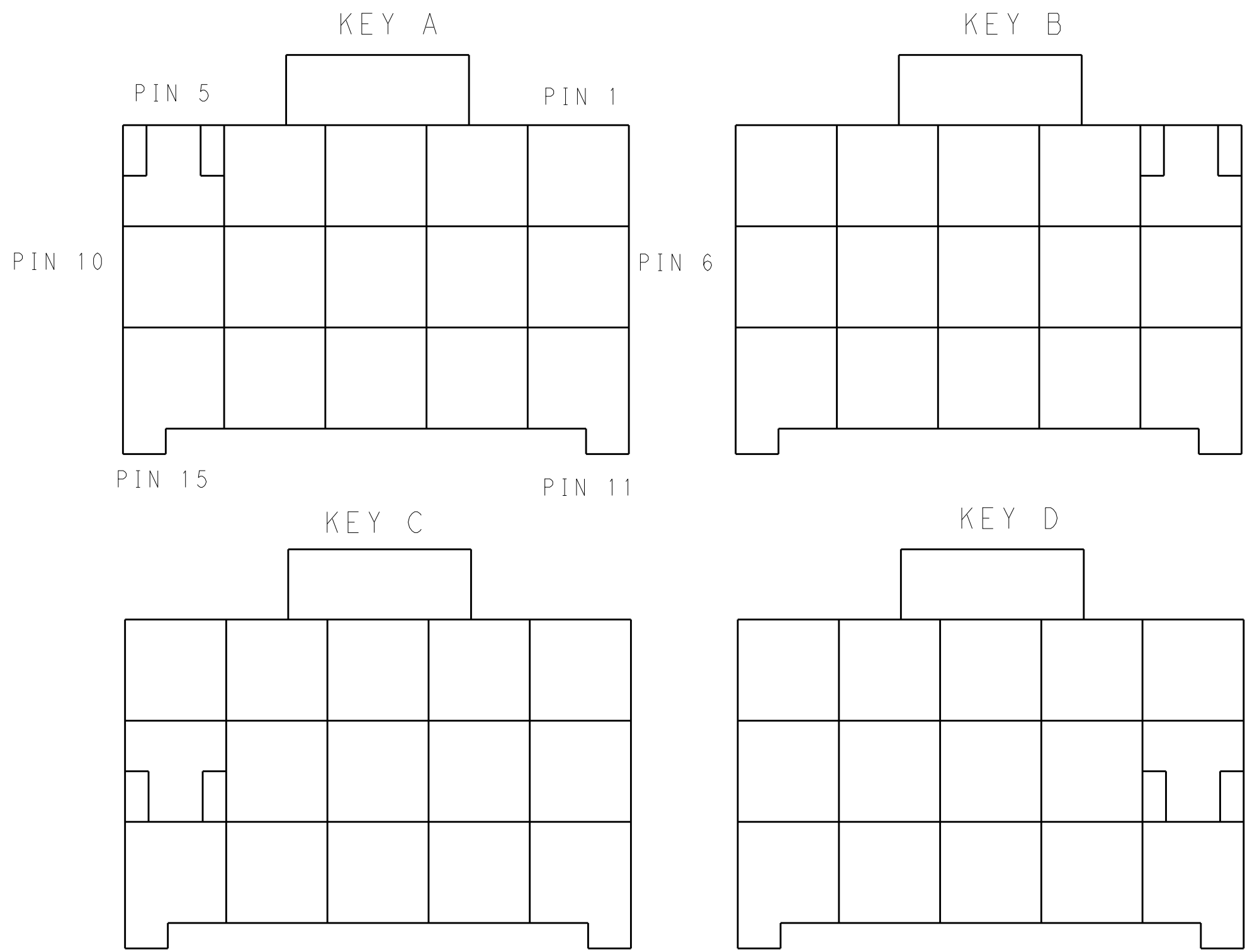
3*5 POSITIONS
