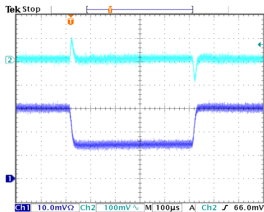
CH1:lout (1A/div) CH2: Vout (3.3V) Load Transient Response
