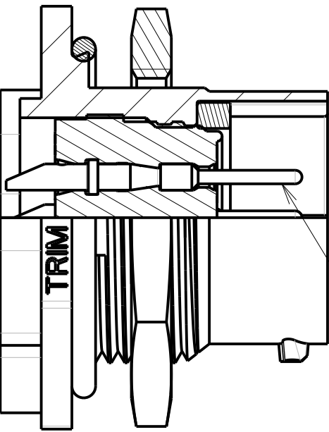
MALE CONNECTOR
