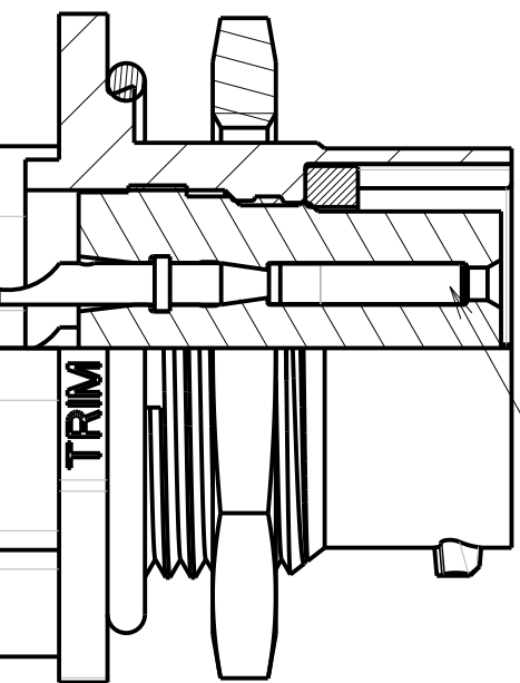
FEMALE CONNECTOR
