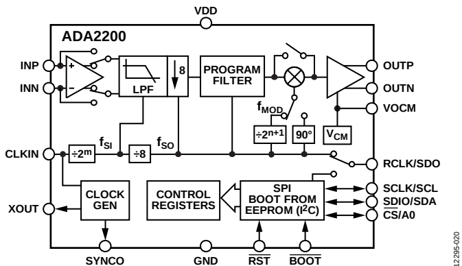
Figure 19. ADA2200 Architecture
