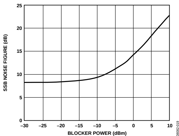
Figure 37. SSB Noise Figure vs. 10 MHz Offset Blocker Power
