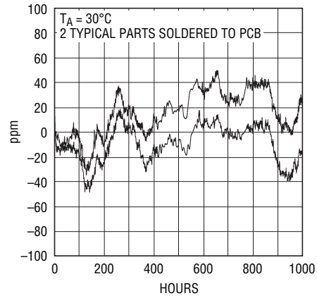
Long-Term Drift
