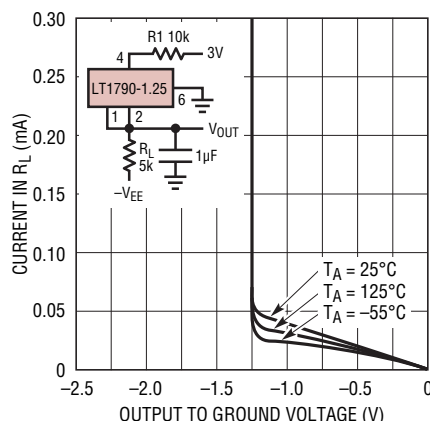
-1.25V Characteristics
