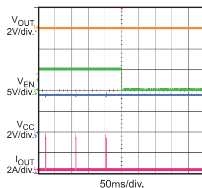
V_{EN} Shutdown with Short
