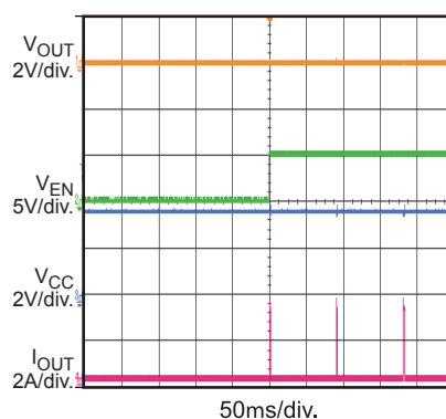
V_{EN} Start-Up with Short
