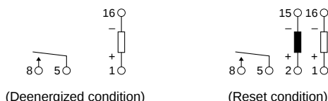
Schematic (Bottom view) Single side stable 2 coil latching
