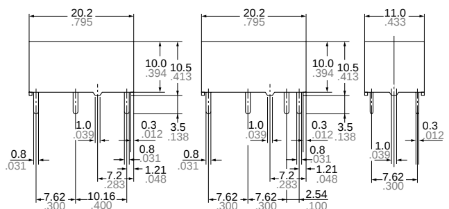
Single side stable External dimensions 2 coil latching
