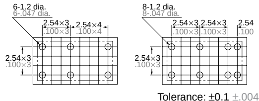
PC board pattern (Bottom view)
