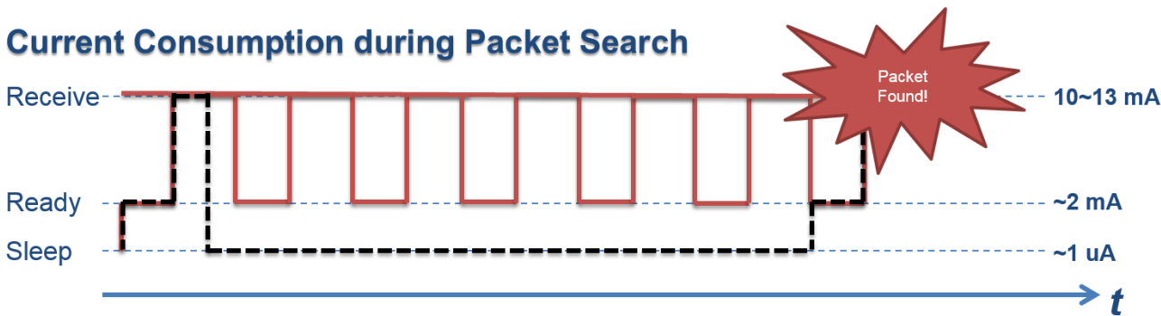
Figure 12. Preamble Sense Mode
