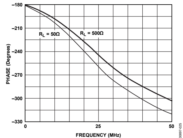
Figure 25. Phase vs. Frequency, Gain = +10
