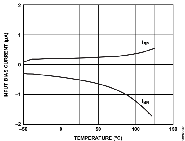
Figure 10. Inverting Input Bias Current ( I_{IN} ) and Noninverting Input Bias Current ( I_{BP} ) vs. Temperature
