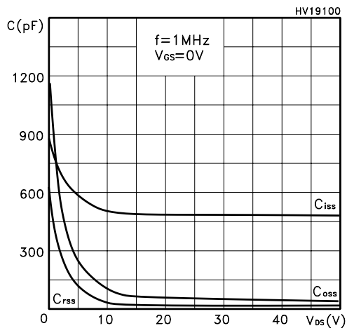
Figure 10: Capacitance variations
