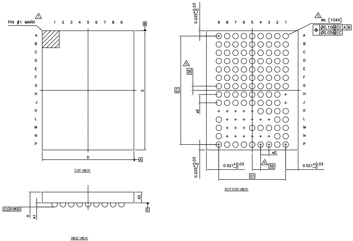
Figure 4. 104-WLCSP 3.8 x 5.0 x 0.65 mm
