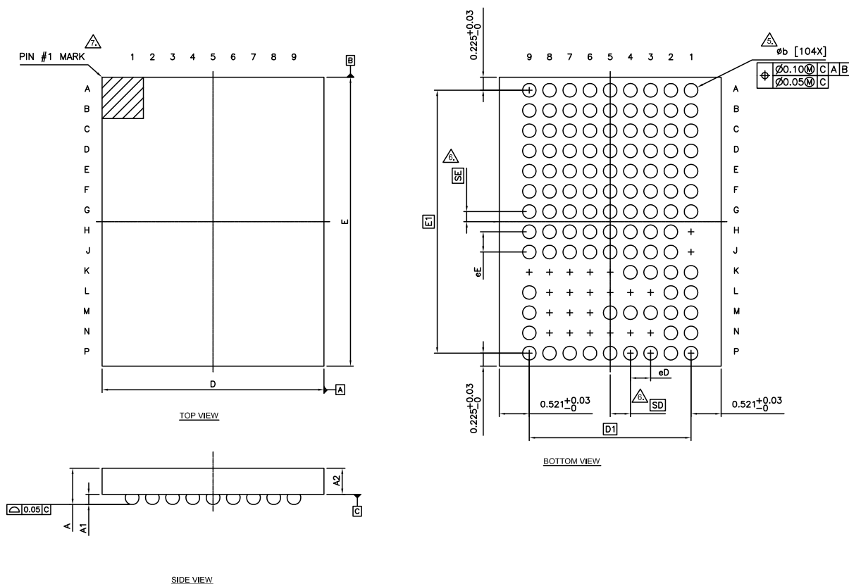
Figure 4. 104-WLCSP 3.8 × 5.0 × 0.65 mm
