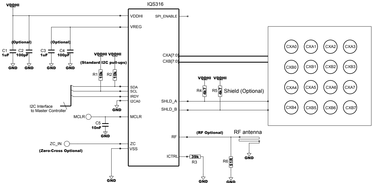
Figure 6.10 Circuit diagram for I²C implementation
