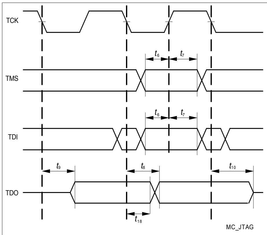
Figure 15 JTAG Timing
