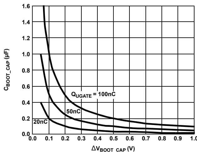
Figure 7. Bootstrap Capacitance vs Boot Ripple Voltage
