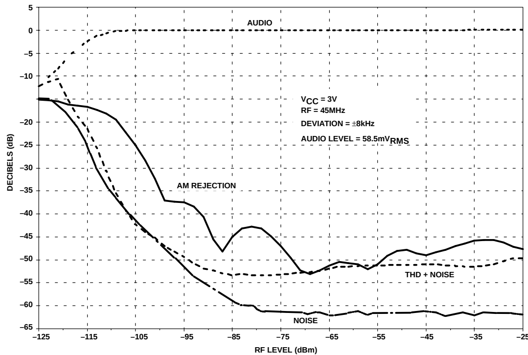
Figure 10. Sensitivity vs RF Level (+25°C)
