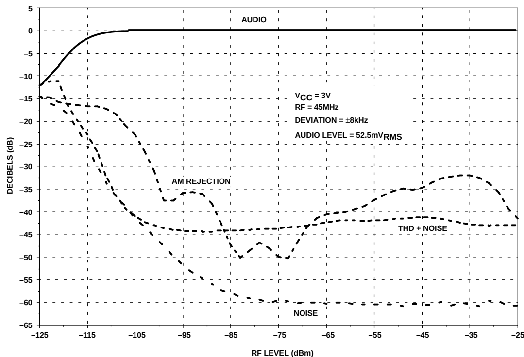
Figure 9. Sensitivity vs RF Level (-40°C)
