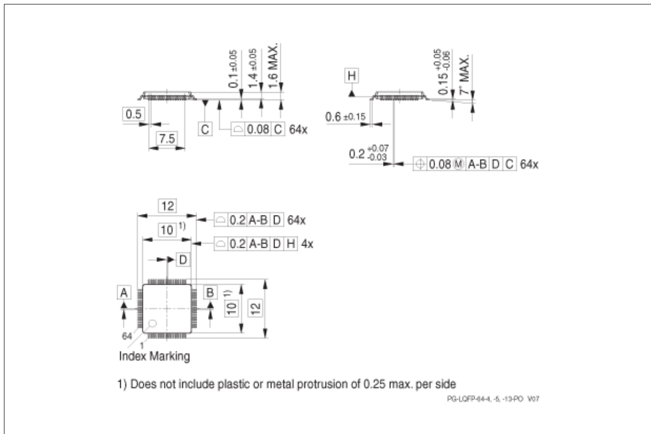
Figure 21 PG-LQFP-64
