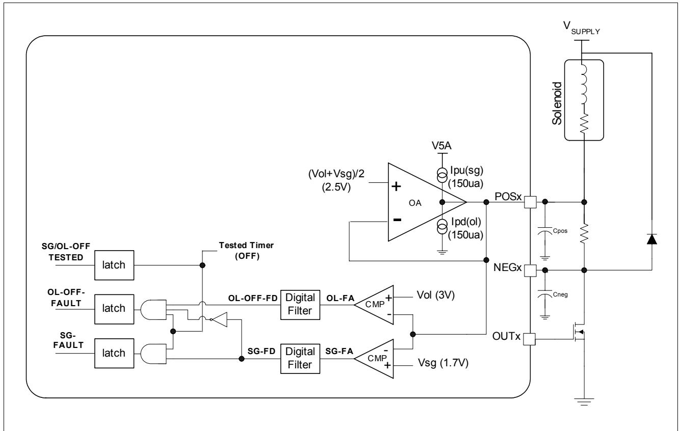
Figure 12 Off-State Diagnostics
