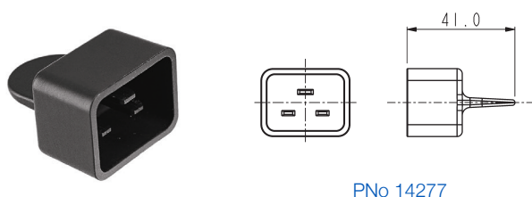
Blanking Cover
