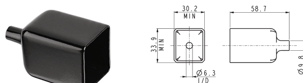
Insulation Boot
