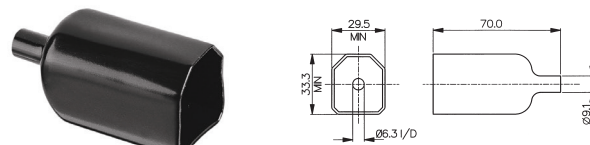
Insulation Boot
