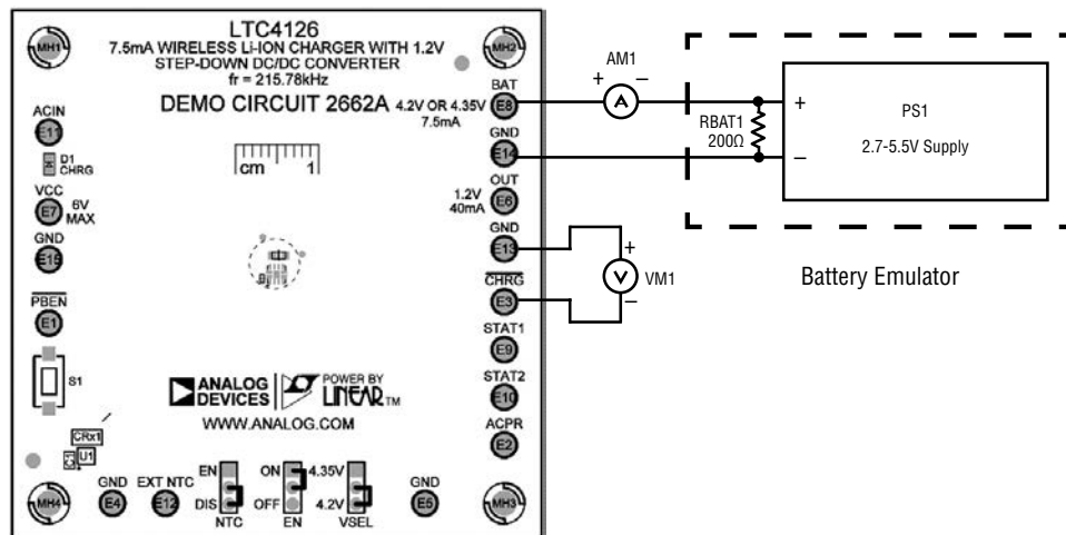
Figure 5. DC2662A Top
