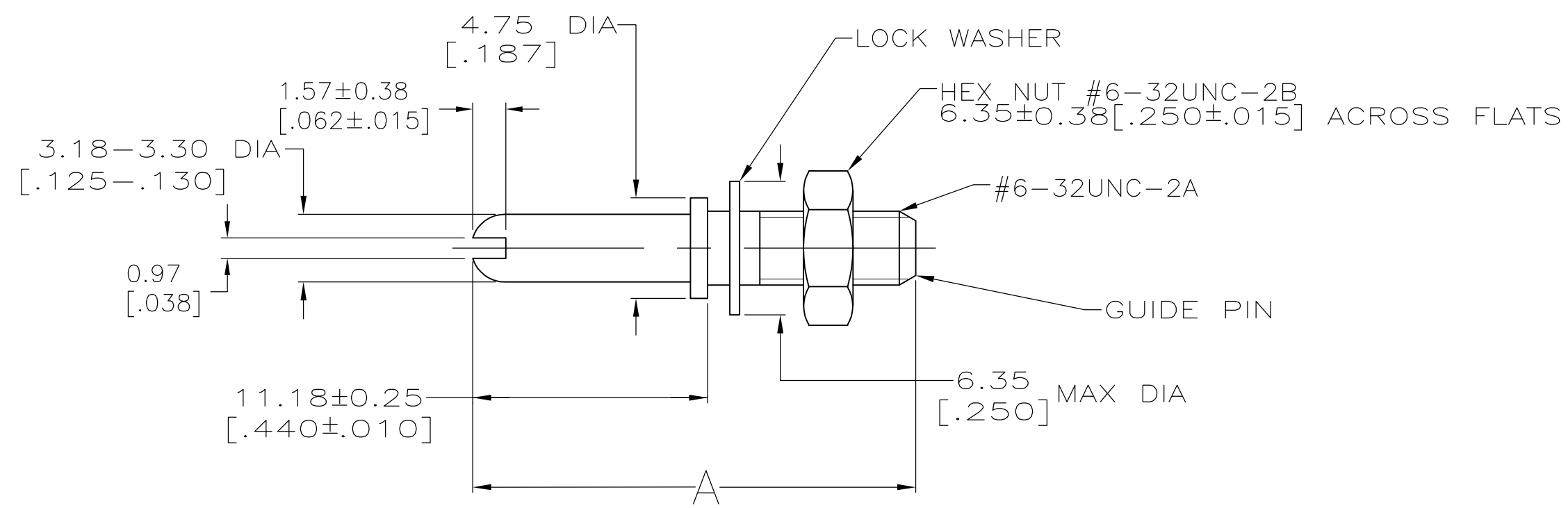
ASSEMBLED VIEW
