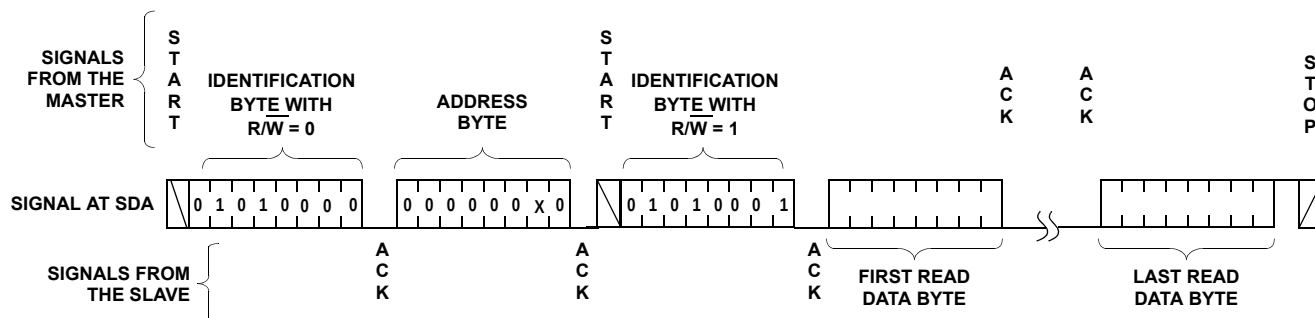
FIGURE 22. READ SEQUENCE
