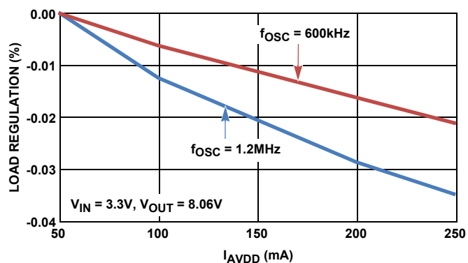
FIGURE 4. AVDD LOAD REGULATION vs I_{AVDD}
