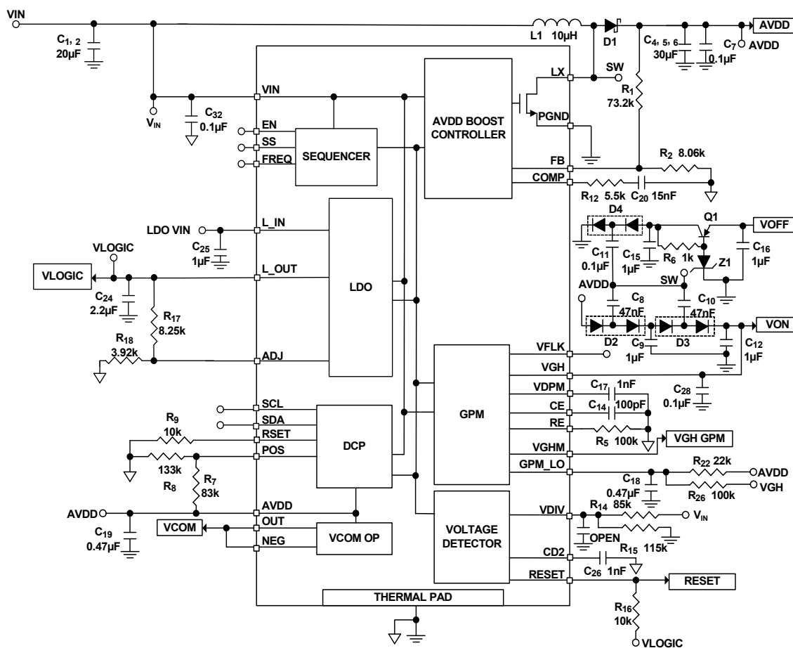
FIGURE 2. APPLICATION DIAGRAM
