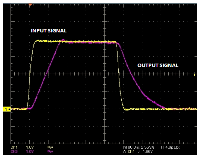
FIGURE 12. V_{COM} RISING SLEW RATE
