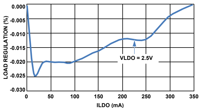
FIGURE 14. LDO LOAD REGULATION vs I_{LDO}
