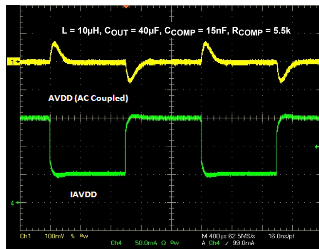
FIGURE 6. BOOST CONVERTER TRANSIENT RESPONSE
