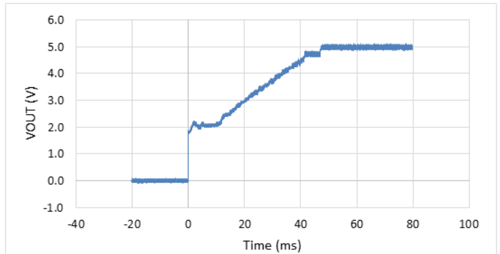
Figure 5.18. 24 V–5 V VOUT Startup vs. Time, 400 mA Load Current
