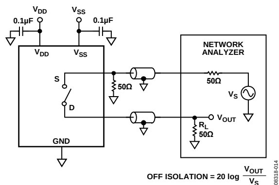
Figure 32. Off Isolation
