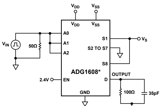
Figure 29. Break-Before-Make Delay, t_{\text{BBM}}
