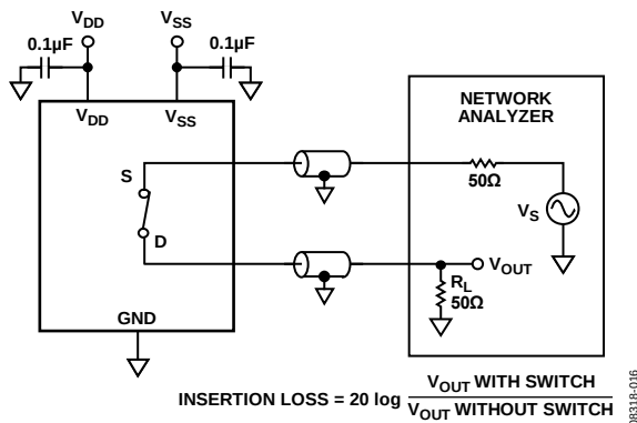
Figure 33. Bandwidth
