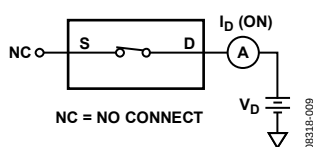
Figure 27. On Leakage
