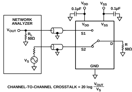
Figure 34. Channel-to-Channel Crosstalk
