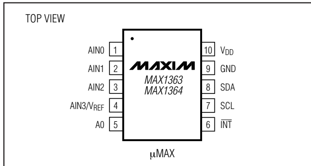
Pin Configuration
