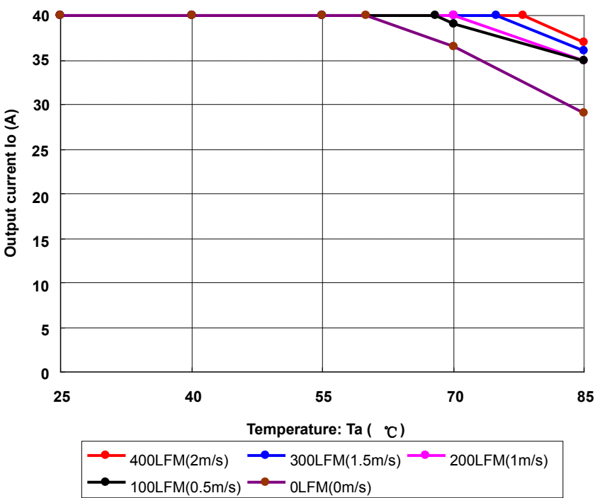
Figure 17 Output power derating, 48Vin, air flowing across the converter from Vin- and Vin+
