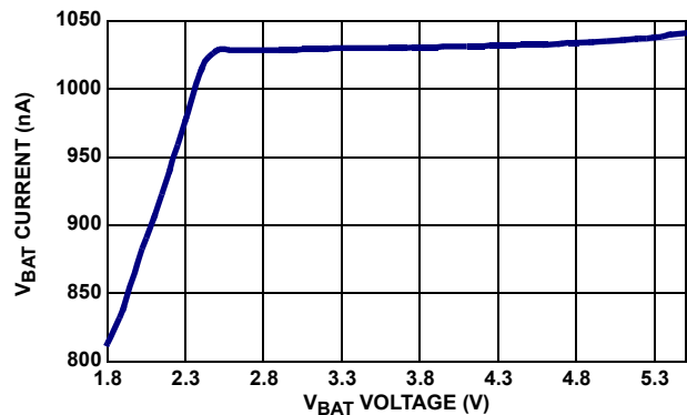
FIGURE 3. I_{BAT} vs V_{BAT}
